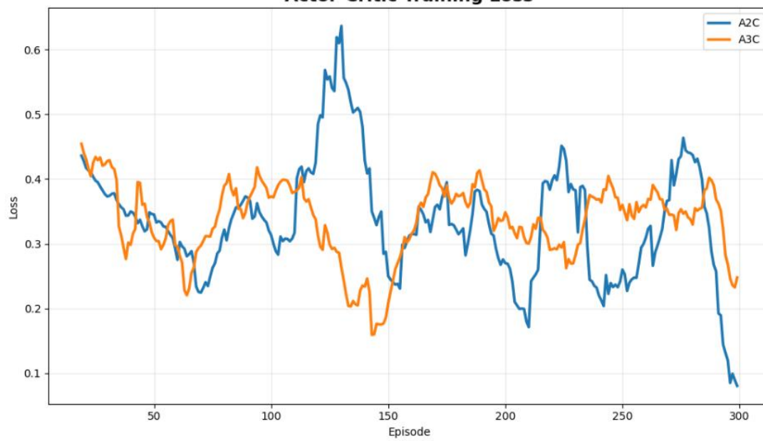
Actor-Critic Training Loss
